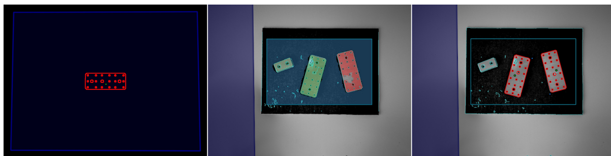
Fig. 6.14: “Template”, “Intermediate Result” and “Result” image streams of the SilhouetteMatch module as shown in the Web GUI for a detection with object_plane_detection set to true
