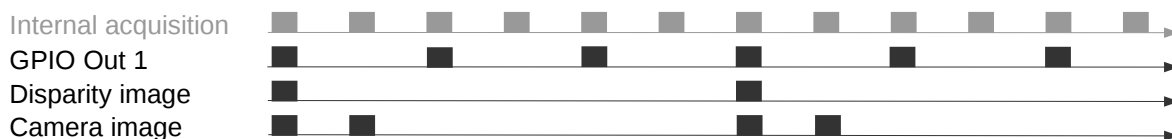
Fig. 6.33: Example of using the ExposureAlternateActive mode for GPIO Out 1 with a user-defined frame rate of 8 Hz. The internal image acquisition is always 25 Hz. GPIO Out 1 is HIGH for the exposure time of every second image. A disparity image is computed for images where Out 1 is HIGH and that are sent out via GigE Vision according to the user-defined frame rate. In ExposureAlternateActive mode, intensity images are always transmitted pairwise: one with GPIO Out 1 HIGH, for which a disparity image might be available, and one with GPIO Out 1 LOW.
