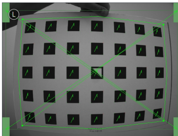
Fig. 6.30: Wrongly holding the grid upside down leads to crossed green lines.
